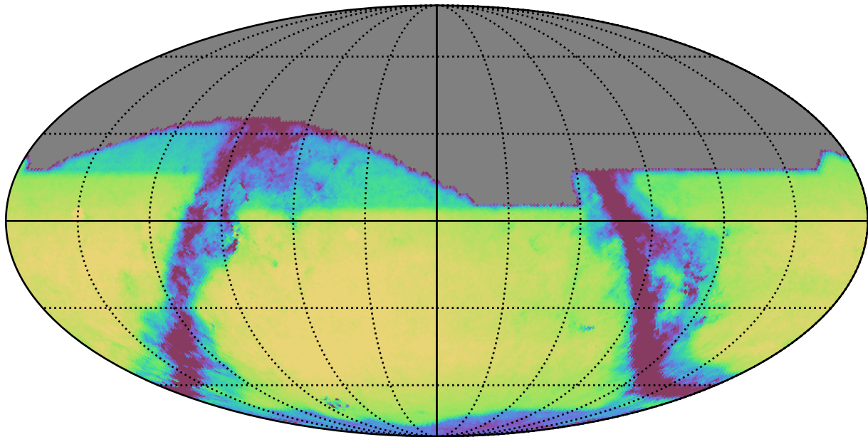
roll_pause_mjdp180_v3.4_10yrs All sky i band: Exgal_CoaddM5
