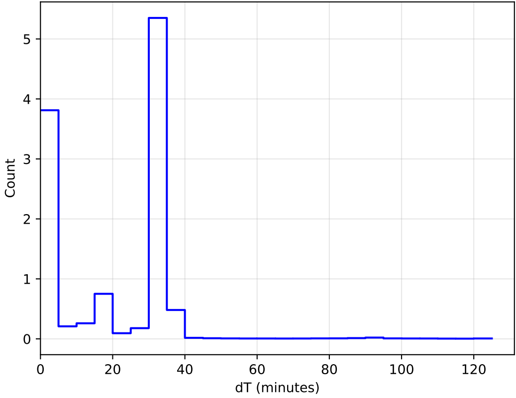
roll_pause_mjdp180_v3.4_10yrs WFD: DeltaT Histogram
