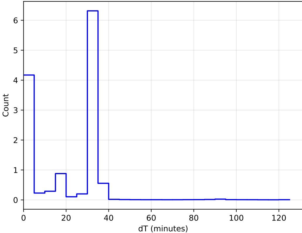
roll_pause_mjdp180_v3.4_10yrs All sky: DeltaT Histogram 1e6
