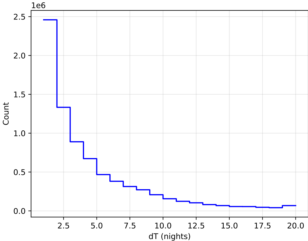
roll_pause_mjdp180_v3.4_10yrs WFD all bands: DeltaNight Histogram
