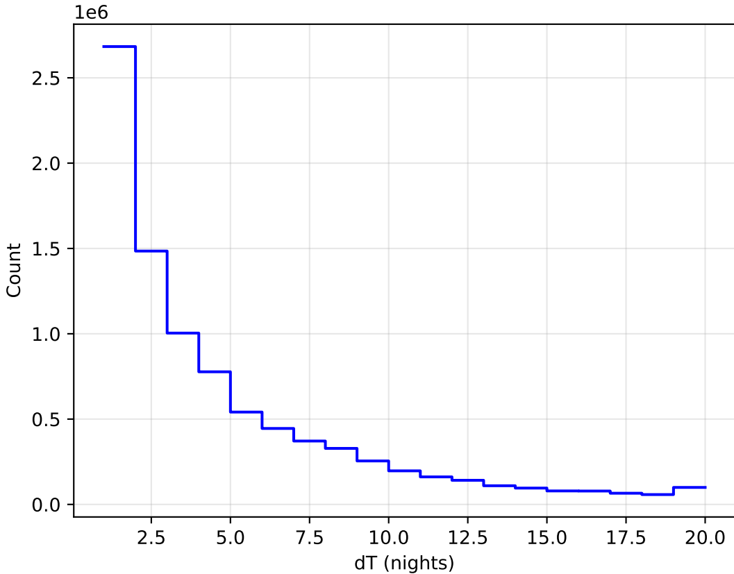
roll_pause_mjdp180_v3.4_10yrs All sky all bands: DeltaNight Histogram
