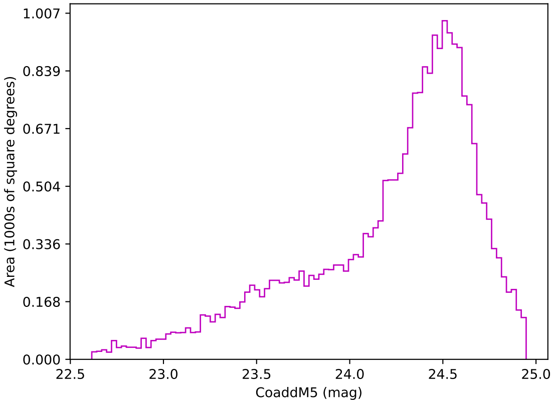
roll_pause_mjdp180_v3.4_10yrs Yr 3-4 z band: CoaddM5
