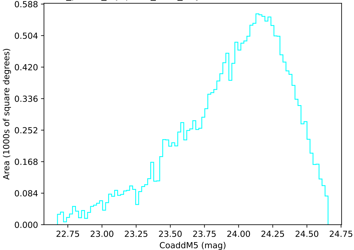
roll_pause_mjdp180_v3.4_10yrs Yr 3-4 u band: CoaddM5
