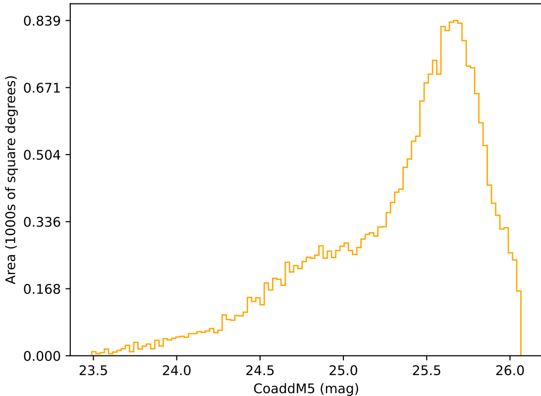
roll_pause_mjdp180_v3.4_10yrs Yr 3-4 r band: CoaddM5
