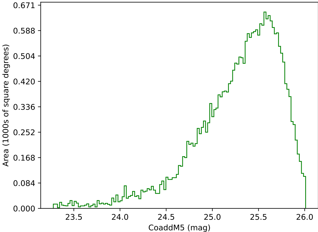
roll_pause_mjdp180_v3.4_10yrs Yr 3-4 g band: CoaddM5
