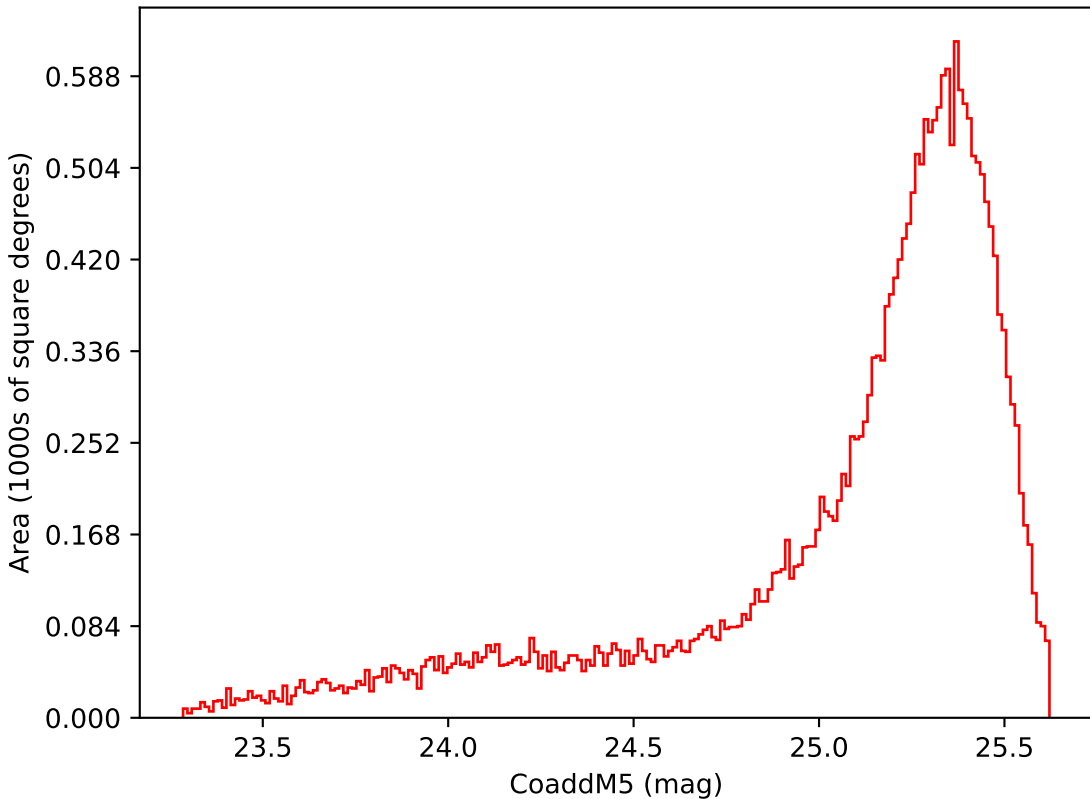
roll_pause_mjdp180_v3.4_10yrs Yr 1 i band: CoaddM5
