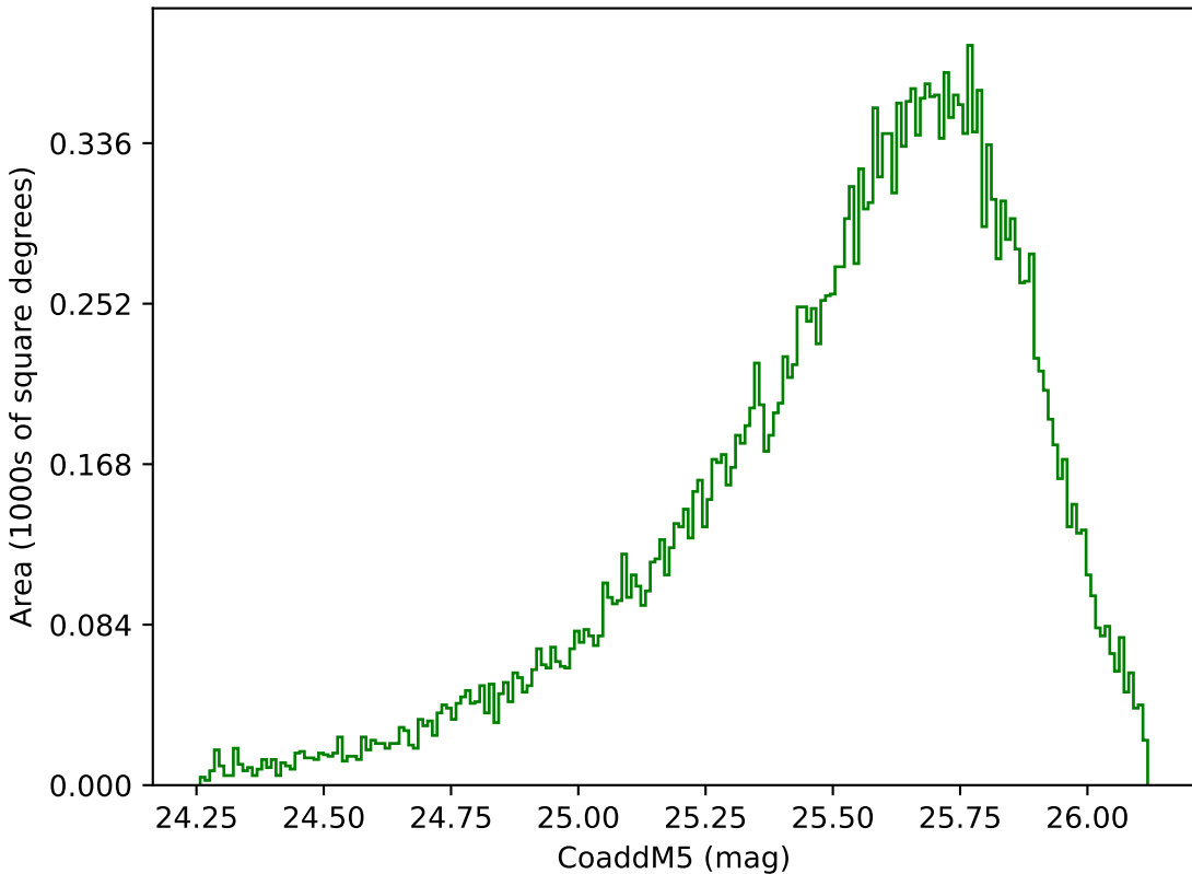
roll_pause_mjdp180_v3.4_10yrs Yr 1 g band: CoaddM5
