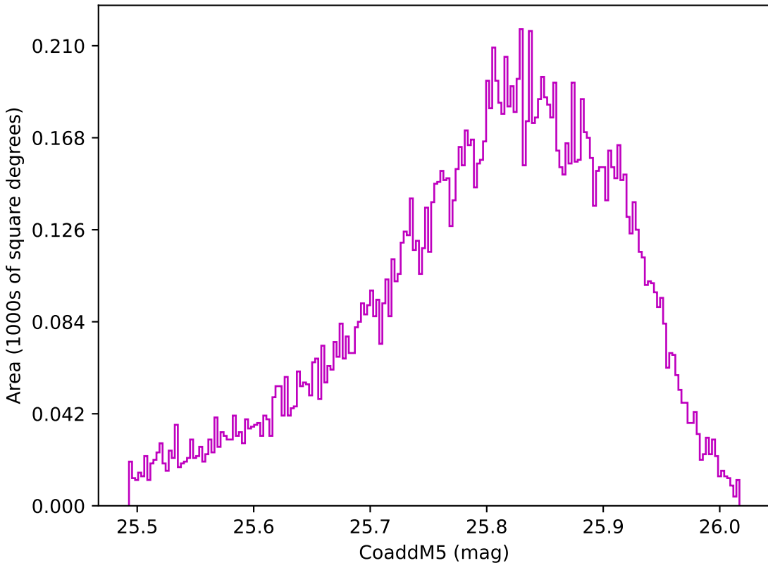
roll_pause_mjdp180_v3.4_10yrs WFD z band: CoaddM5
