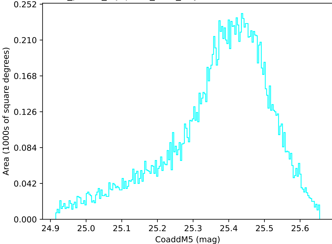
roll_pause_mjdp180_v3.4_10yrs WFD u band: CoaddM5
