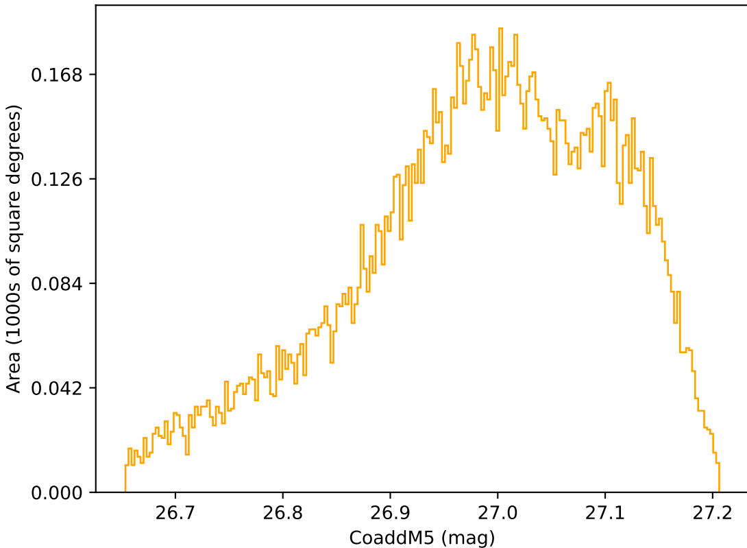
roll_pause_mjdp180_v3.4_10yrs WFD r band: CoaddM5
