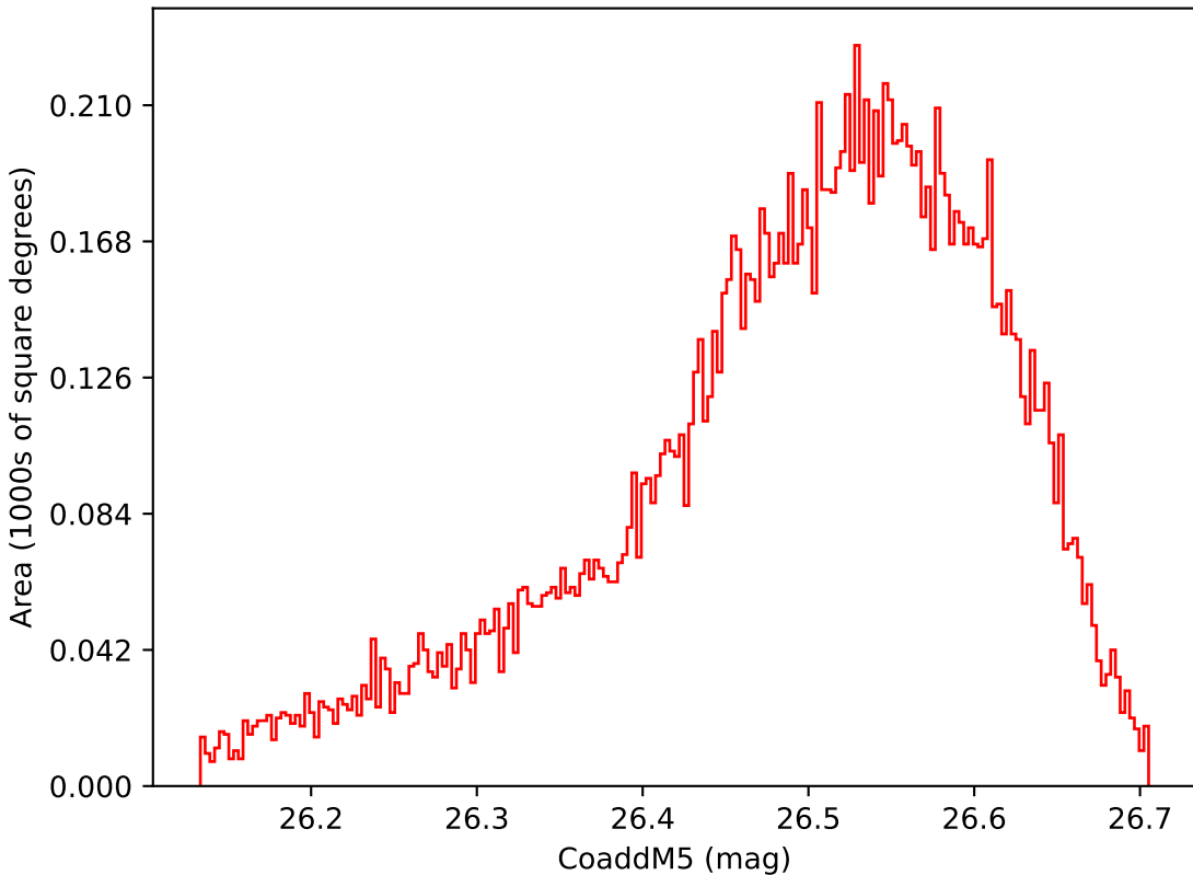
roll_pause_mjdp180_v3.4_10yrs WFD i band: CoaddM5
