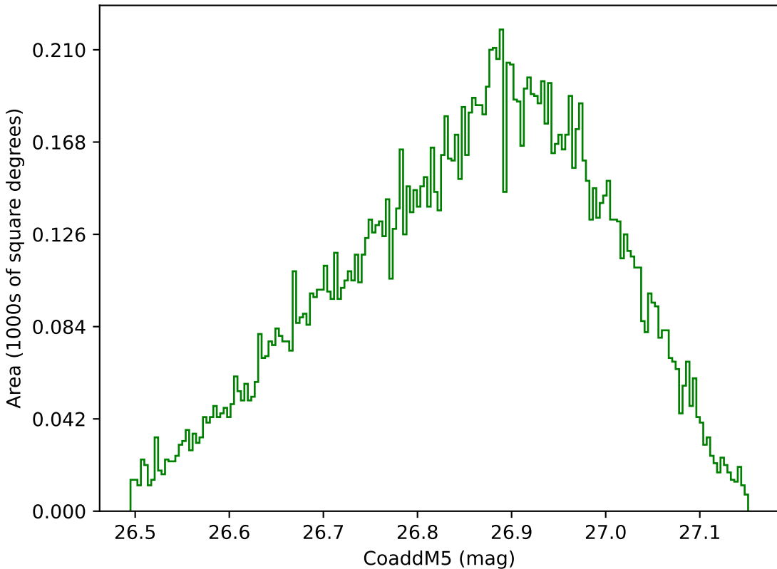
roll_pause_mjdp180_v3.4_10yrs WFD g band: CoaddM5
