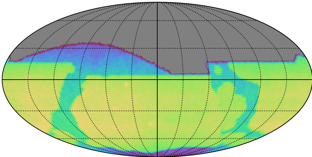
roll_pause_mjdp180_v3.4_10yrs All sky z band: CoaddM5
