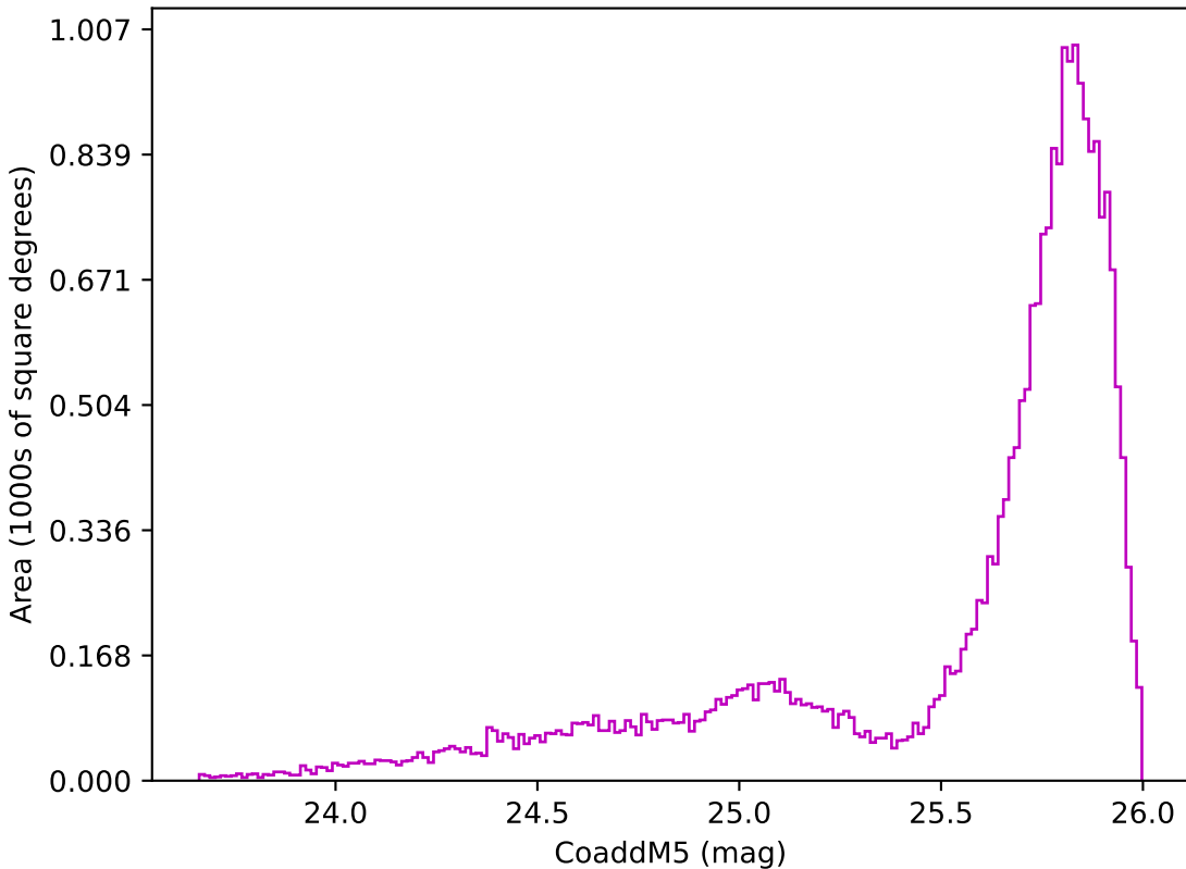
roll_pause_mjdp180_v3.4_10yrs All sky z band: CoaddM5
