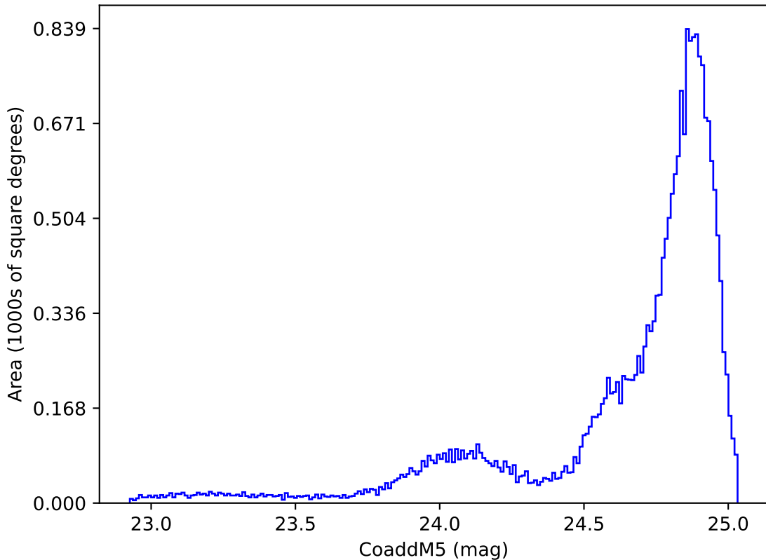
roll_pause_mjdp180_v3.4_10yrs All sky y band: CoaddM5
