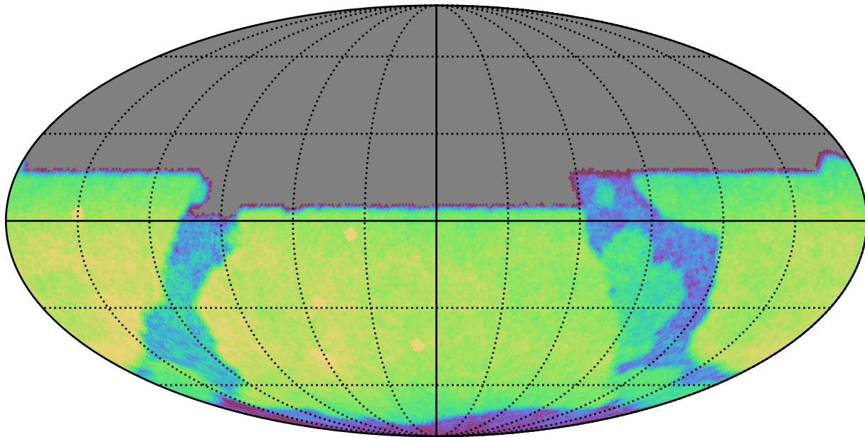
roll_pause_mjdp180_v3.4_10yrs All sky u band: CoaddM5
