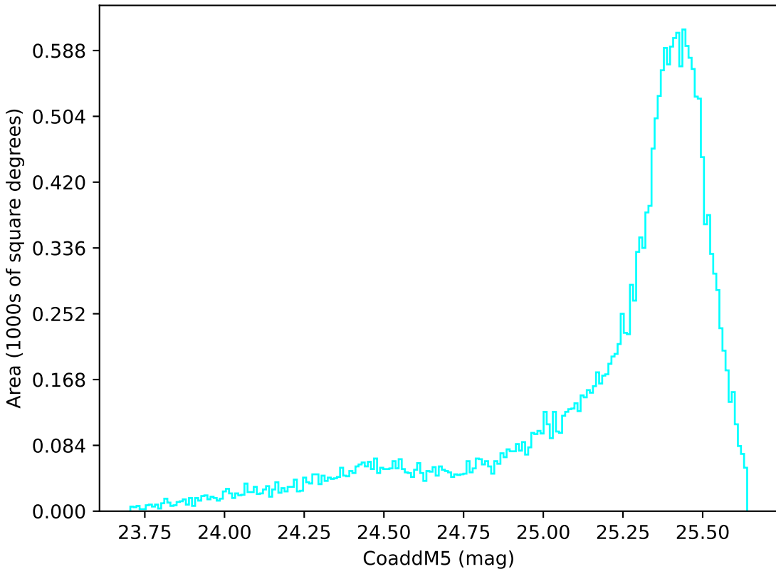
roll_pause_mjdp180_v3.4_10yrs All sky u band: CoaddM5
