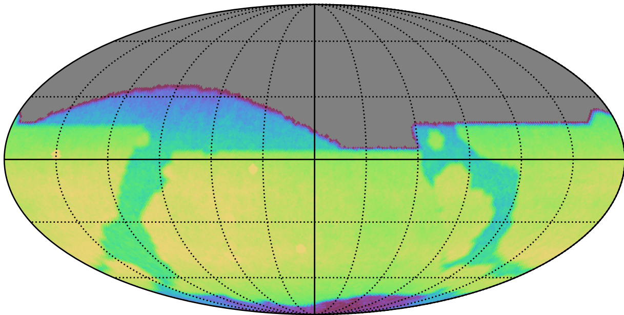
roll_pause_mjdp180_v3.4_10yrs All sky r band: CoaddM5
