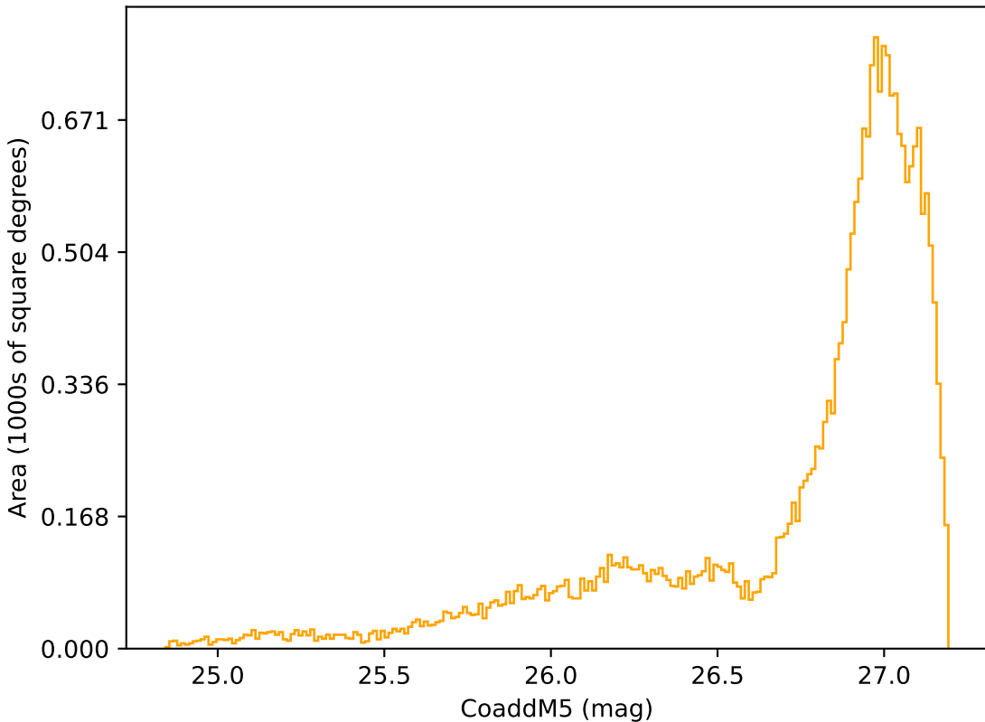
roll_pause_mjdp180_v3.4_10yrs All sky r band: CoaddM5
