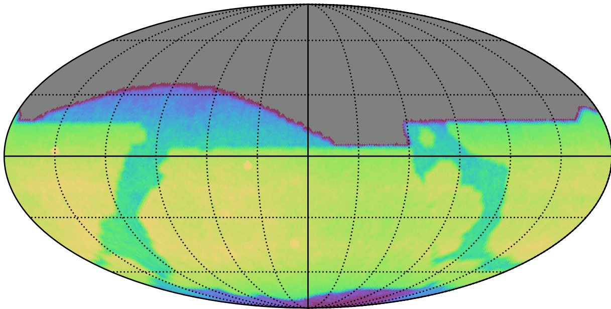
roll_pause_mjdp180_v3.4_10yrs All sky i band: CoaddM5
