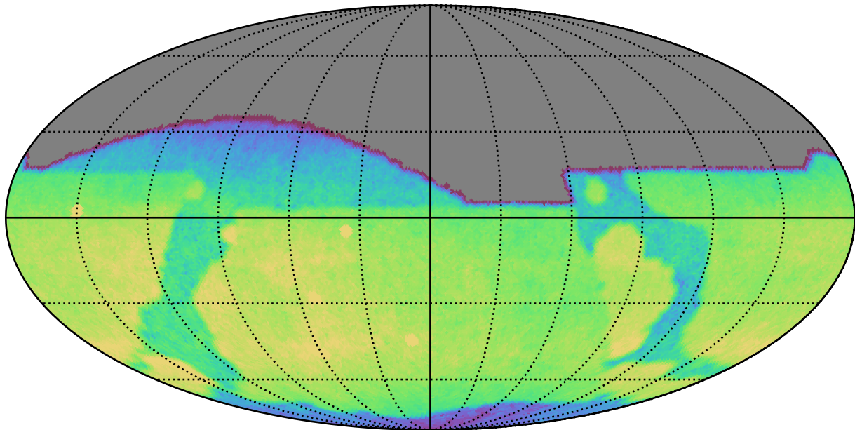
roll_pause_mjdp180_v3.4_10yrs All sky g band: CoaddM5
