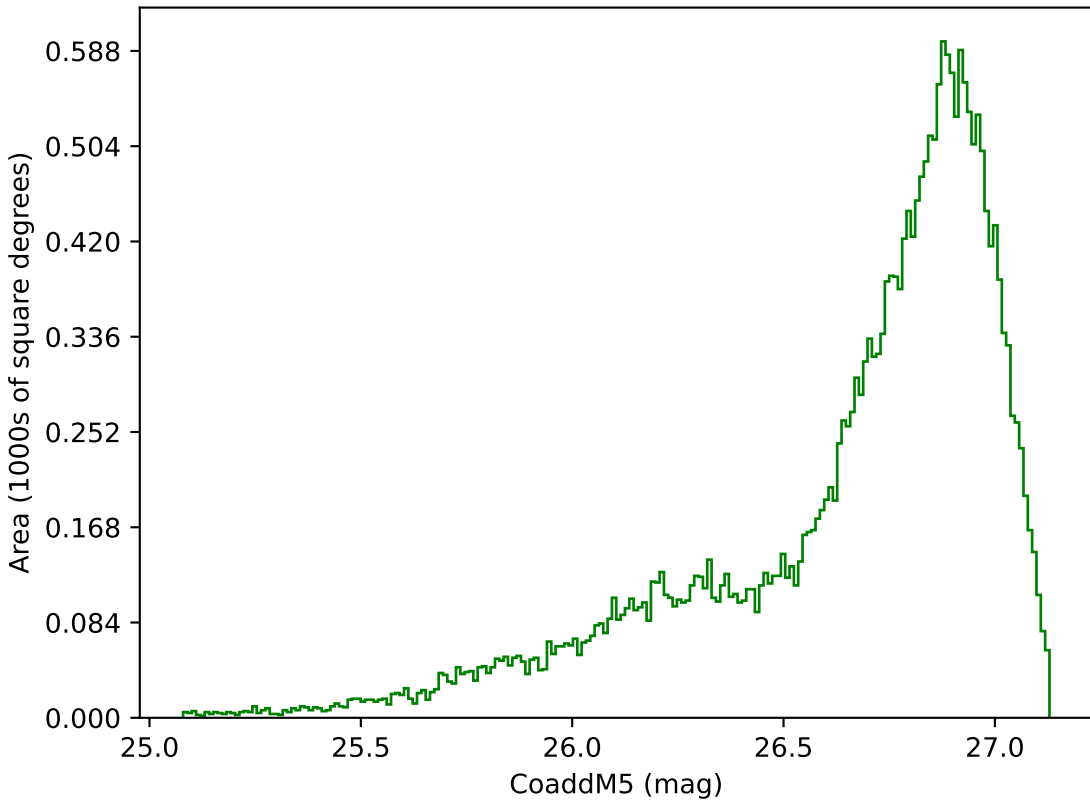
roll_pause_mjdp180_v3.4_10yrs All sky g band: CoaddM5
