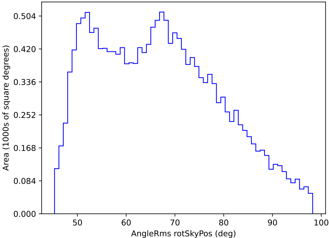
roll_pause_mjdp180_v3.4_10yrs WFD r band: AngleRms rotSkyPos
