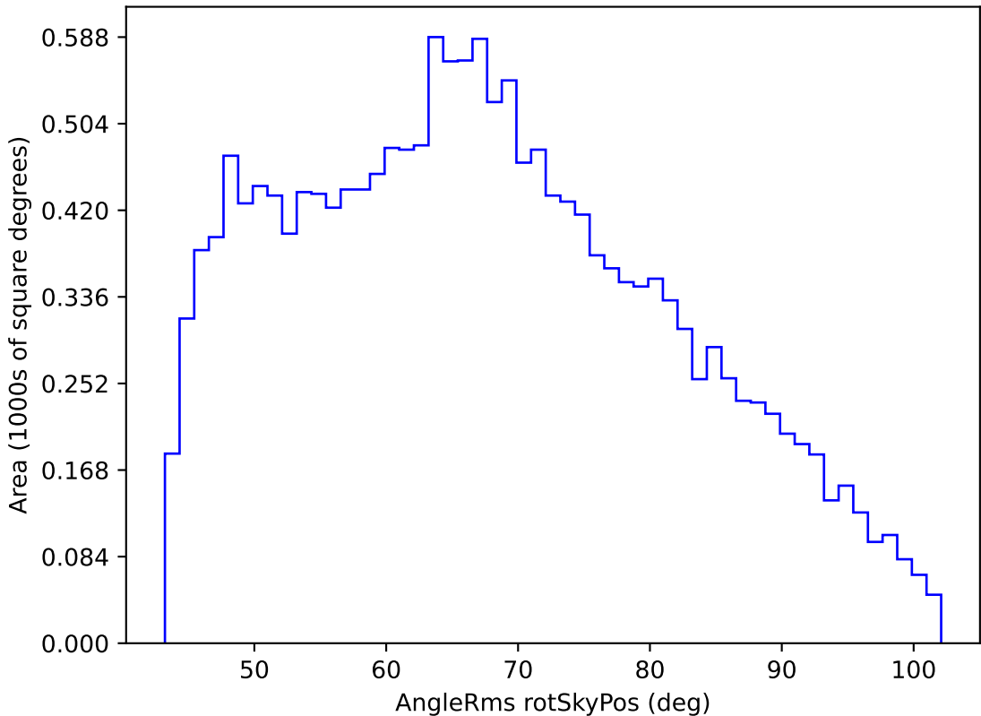
roll_pause_mjdp180_v3.4_10yrs WFD g band: AngleRms rotSkyPos
