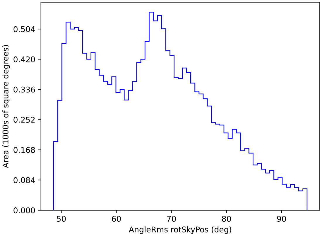
roll_pause_mjdp180_v3.4_10yrs WFD all bands: AngleRms rotSkyPos
