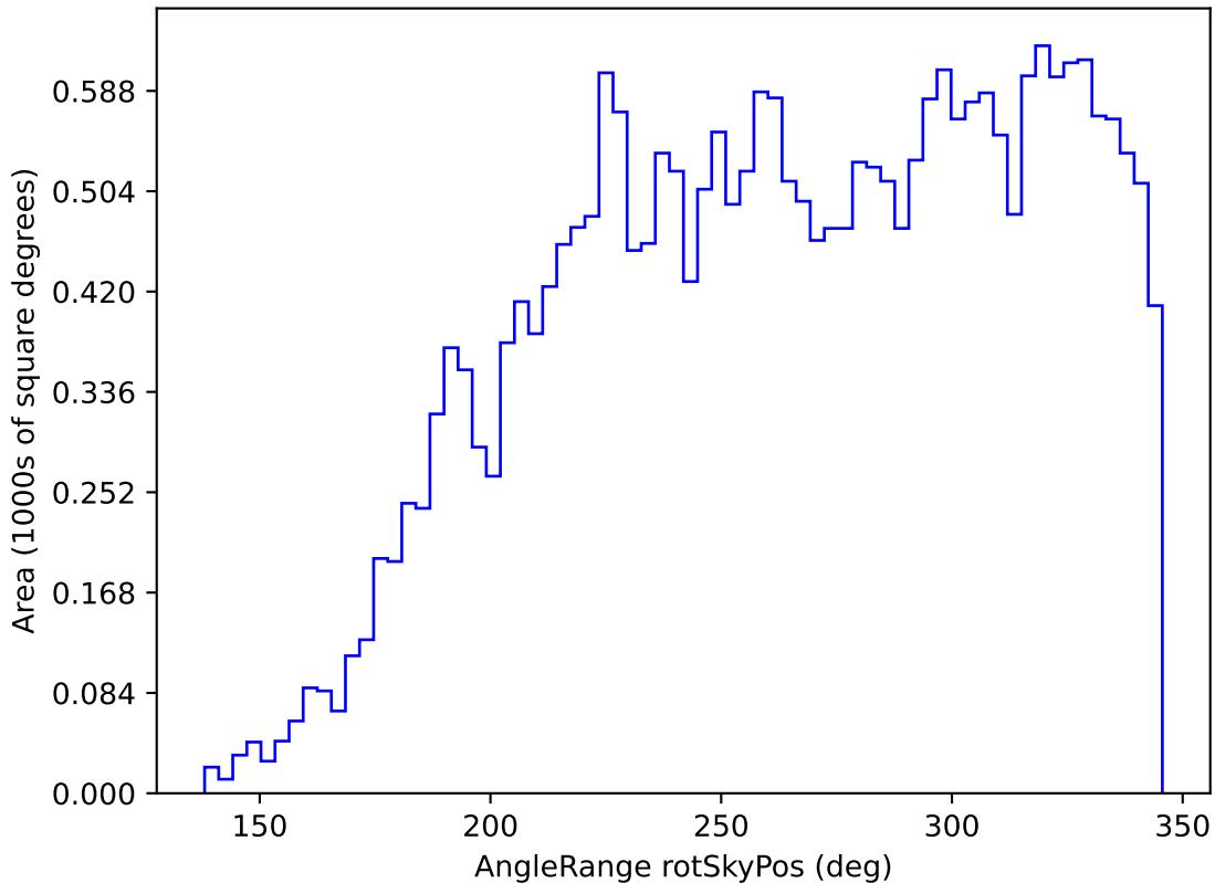
roll_pause_mjdp180_v3.4_10yrs All sky i band: AngleRange rotSkyPos
