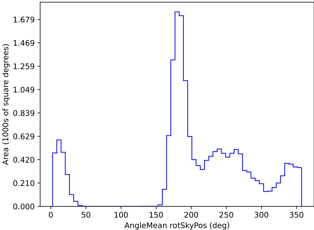
roll_pause_mjdp180_v3.4_10yrs WFD z band: AngleMean rotSkyPos
