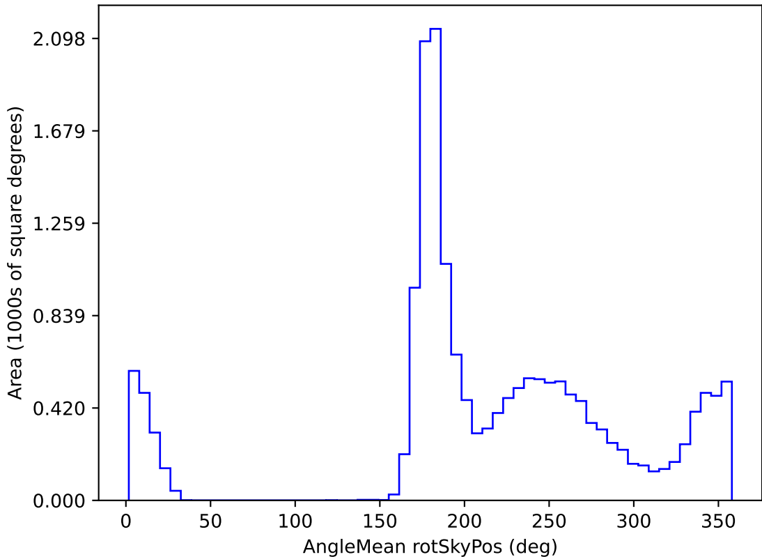
roll_pause_mjdp180_v3.4_10yrs WFD i band: AngleMean rotSkyPos
