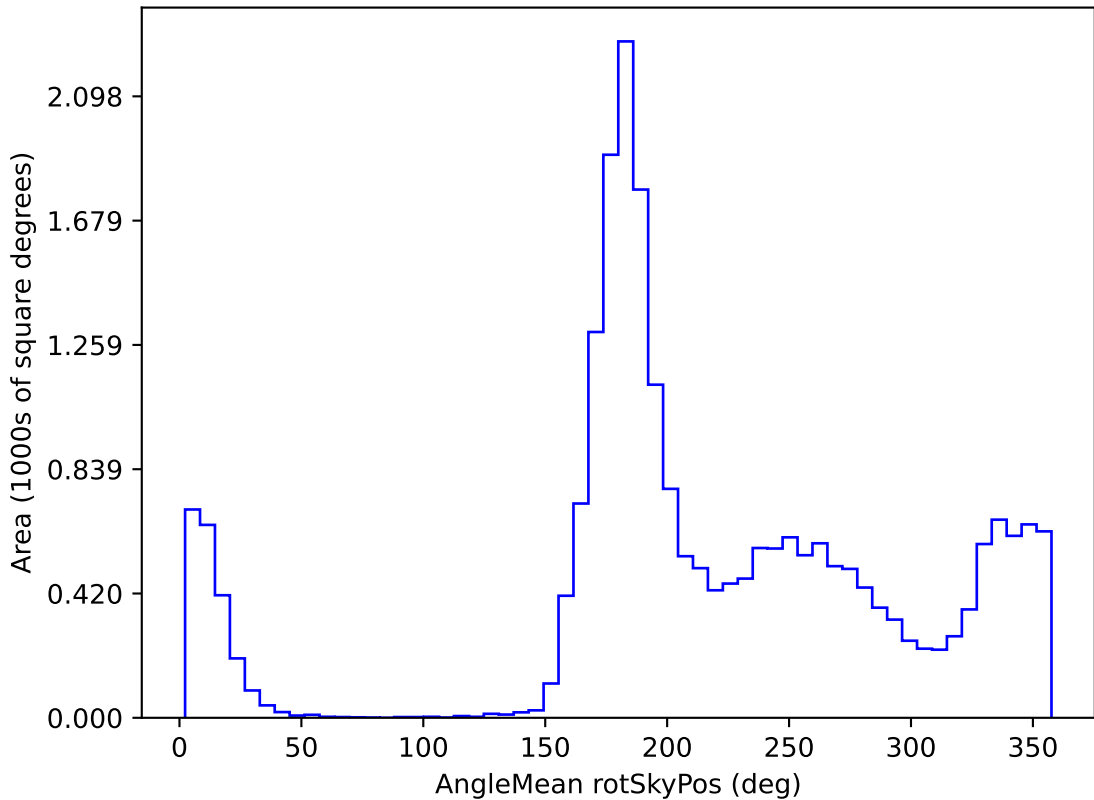
roll_pause_mjdp180_v3.4_10yrs All sky y band: AngleMean rotSkyPos
