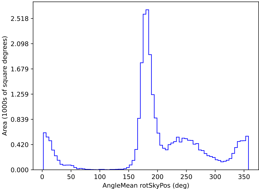
roll_pause_mjdp180_v3.4_10yrs All sky i band: AngleMean rotSkyPos
