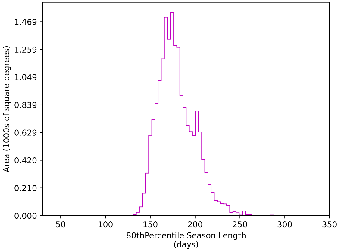
roll_pause_mjdp180_v3.4_10yrs WFD z band: 80thPercentile Season Length
