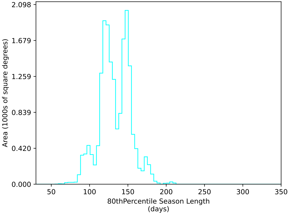
roll_pause_mjdp180_v3.4_10yrs WFD u band: 80thPercentile Season Length
