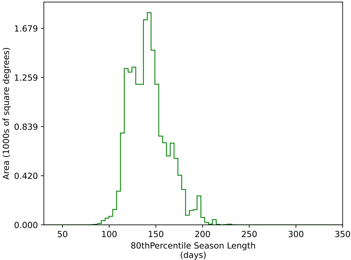
roll_pause_mjdp180_v3.4_10yrs WFD g band: 80thPercentile Season Length
