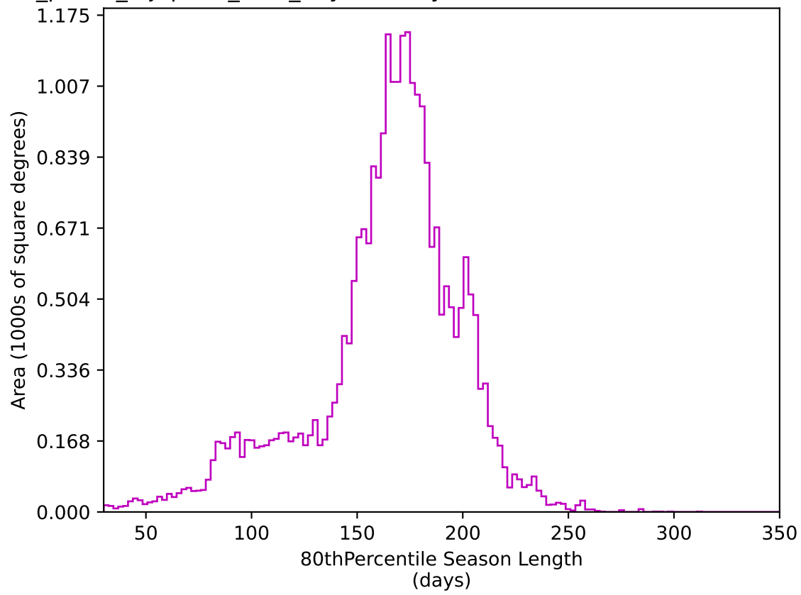
roll_pause_mjdp180_v3.4_10yrs All sky z band: 80thPercentile Season Length
