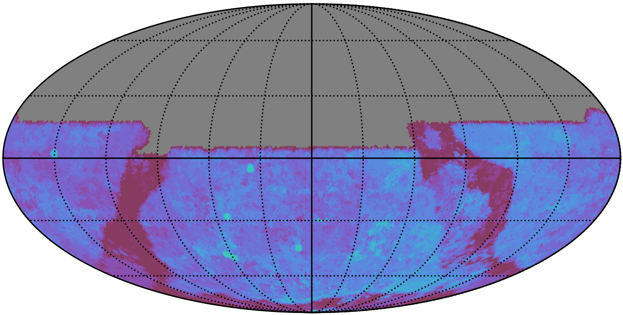
roll_pause_mjdp180_v3.4_10yrs All sky u band: 80thPercentile Season Length
