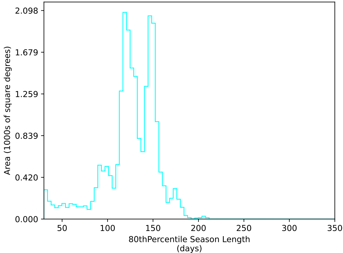
roll_pause_mjdp180_v3.4_10yrs All sky u band: 80thPercentile Season Length
