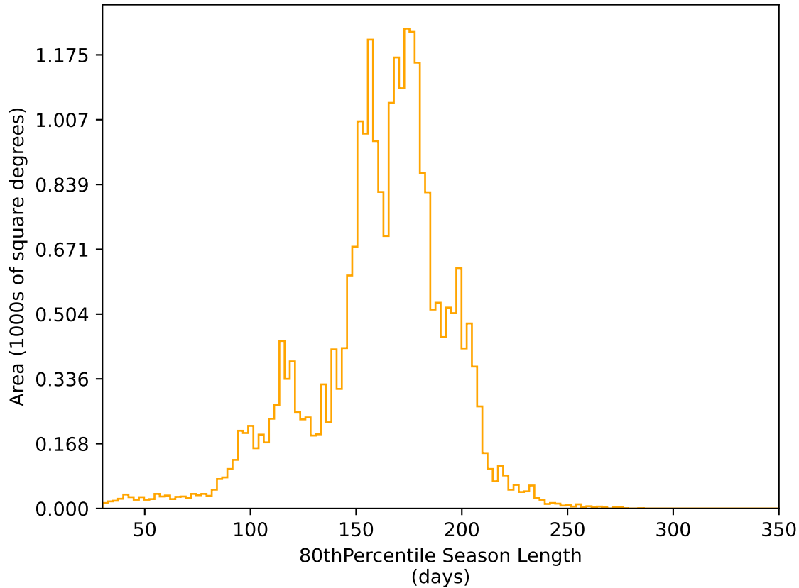
roll_pause_mjdp180_v3.4_10yrs All sky r band: 80thPercentile Season Length
