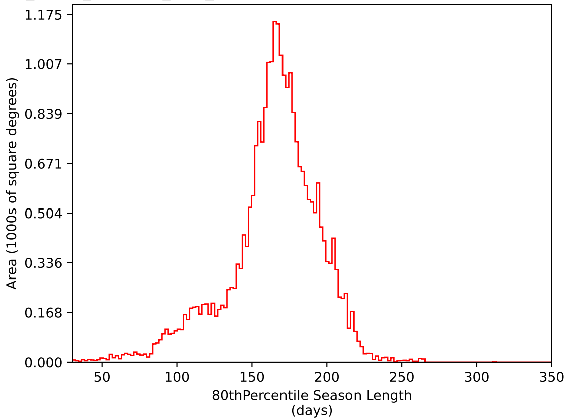
roll_pause_mjdp180_v3.4_10yrs All sky i band: 80thPercentile Season Length
