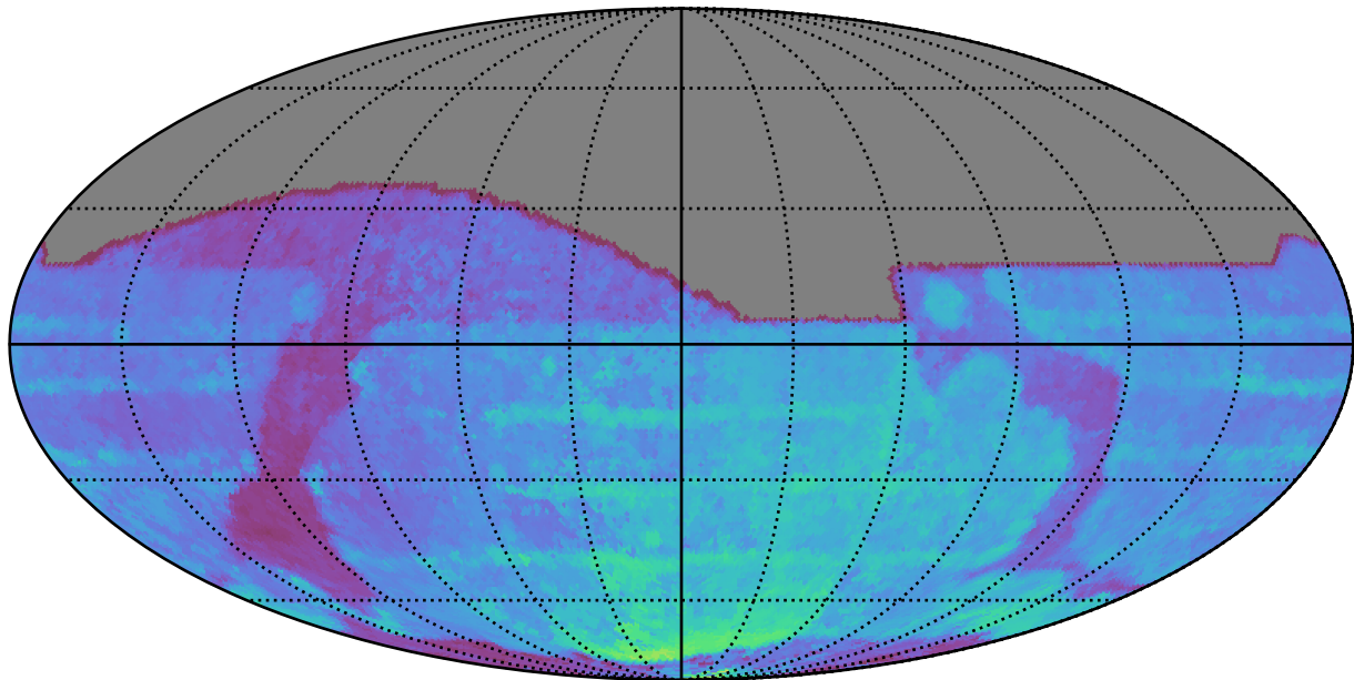
roll_pause_mjdp180_v3.4_10yrs All sky all bands: 80thPercentile Season Length
