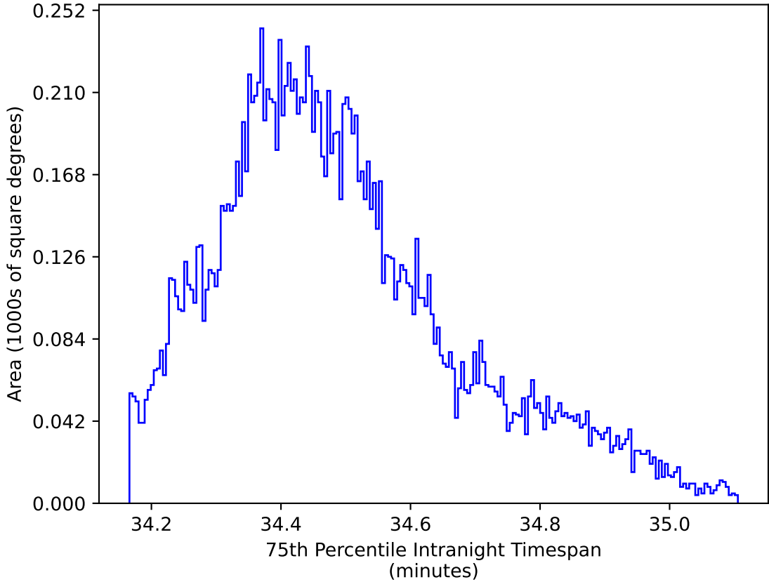
roll_pause_mjdp180_v3.4_10yrs WFD zy bands: 75th Percentile Intranight Timespan
