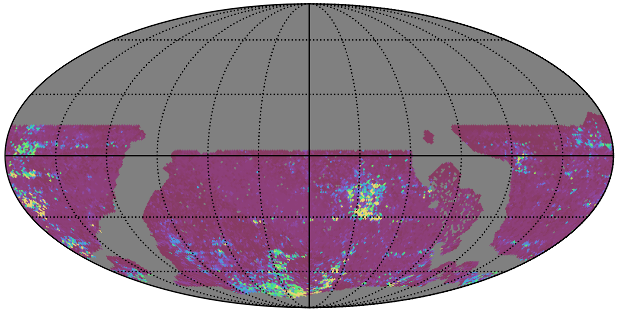
roll_pause_mjdp180_v3.4_10yrs WFD z band: 75th Percentile Intranight Timespan
