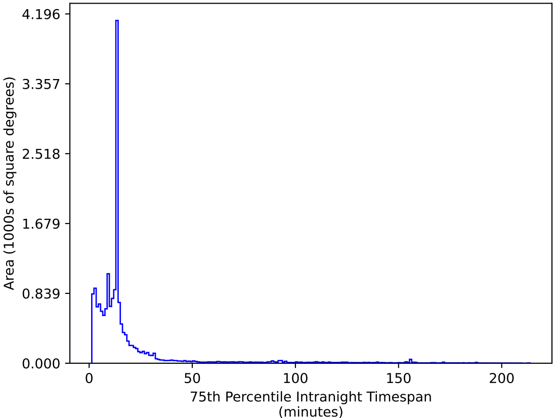
roll_pause_mjdp180_v3.4_10yrs WFD z band: 75th Percentile Intranight Timespan
