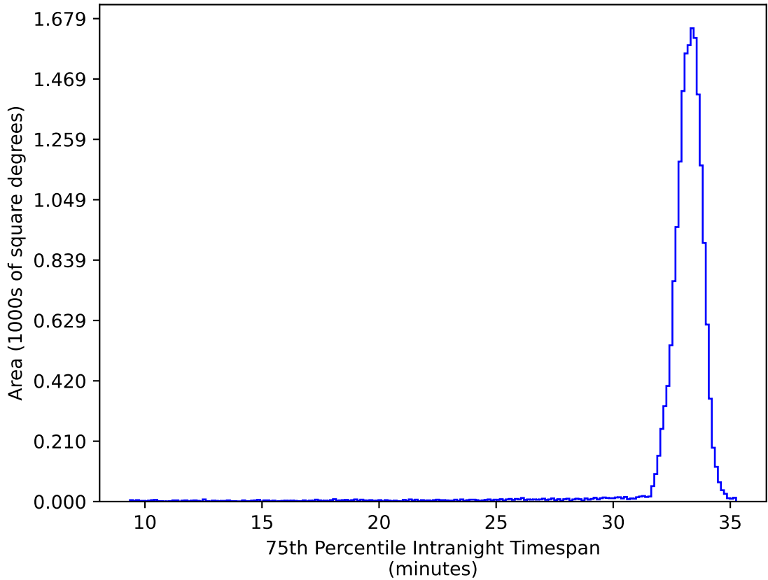
roll_pause_mjdp180_v3.4_10yrs WFD ug bands: 75th Percentile Intranight Timespan
