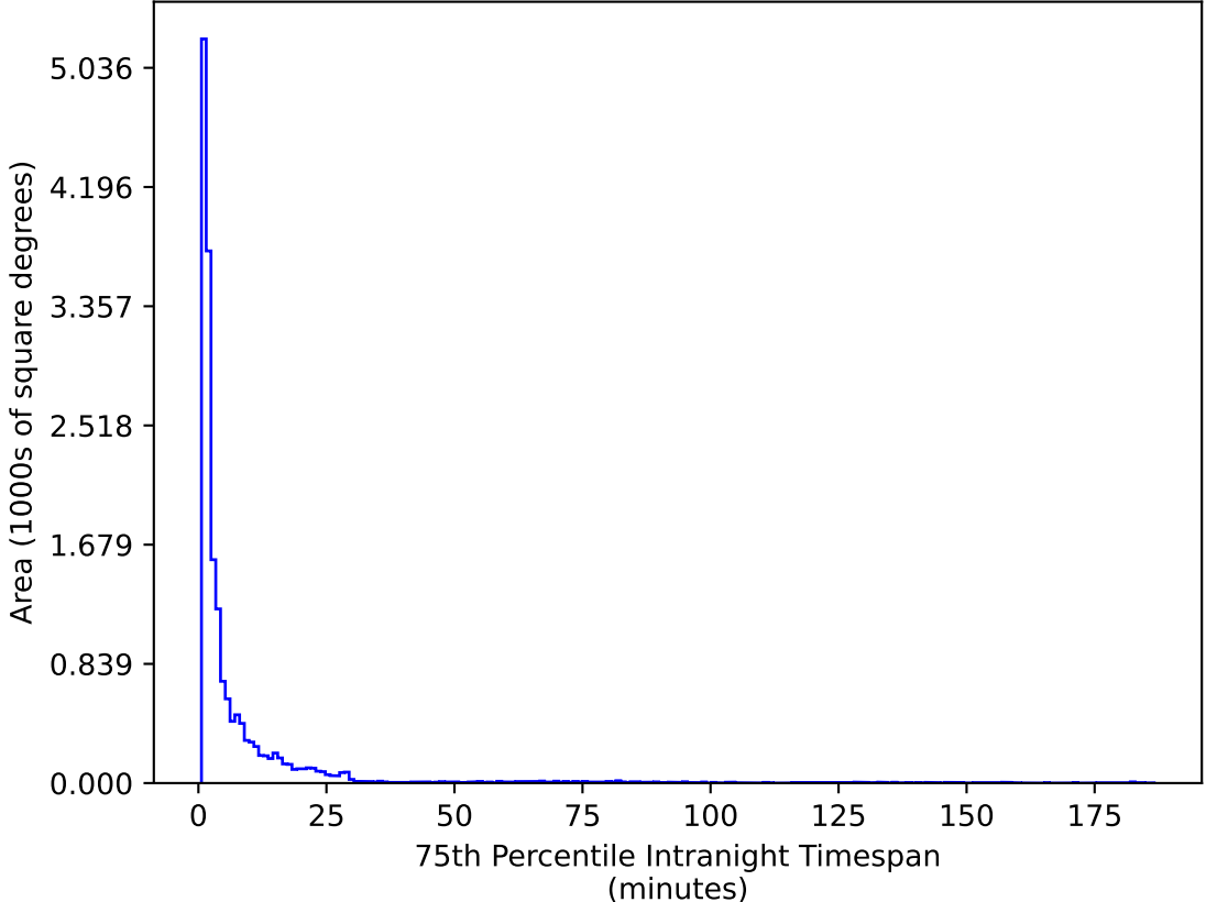
roll_pause_mjdp180_v3.4_10yrs WFD u band: 75th Percentile Intranight Timespan
