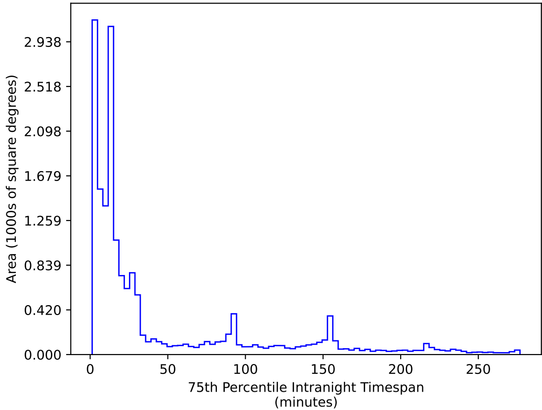
roll_pause_mjdp180_v3.4_10yrs WFD r band: 75th Percentile Intranight Timespan
