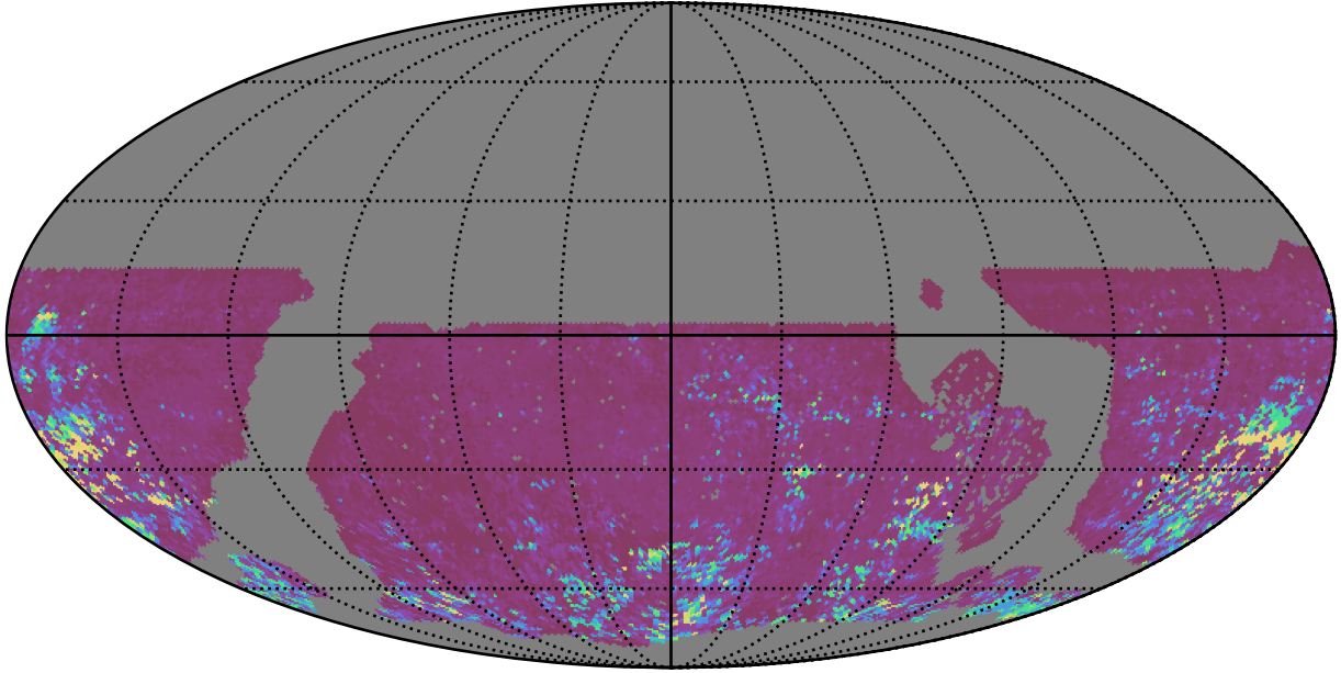
roll_pause_mjdp180_v3.4_10yrs WFD i band: 75th Percentile Intranight Timespan
